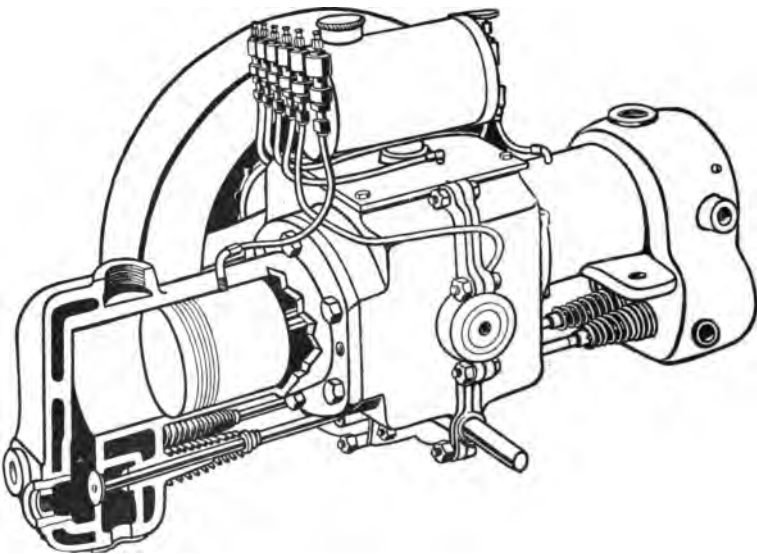
FIG. 397.—Section of the Ford Double-Opposed-Cylinder Horizontal Engine, showing oil leads to the various points from the lubricator operated by compressed air from the crank case.
